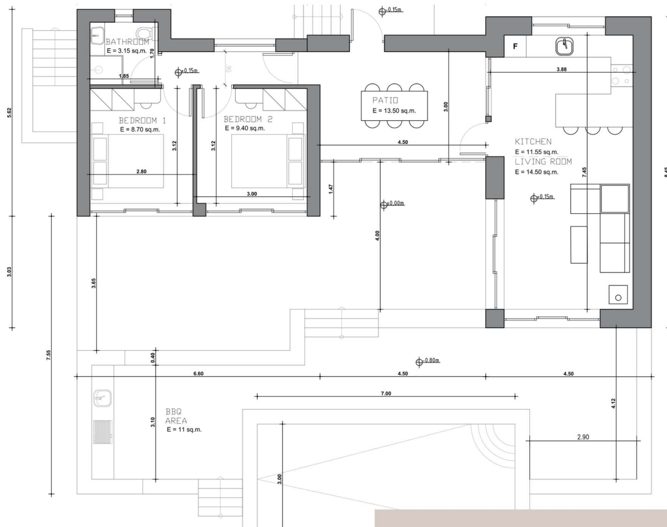
PLAN PLAIN-PIED
