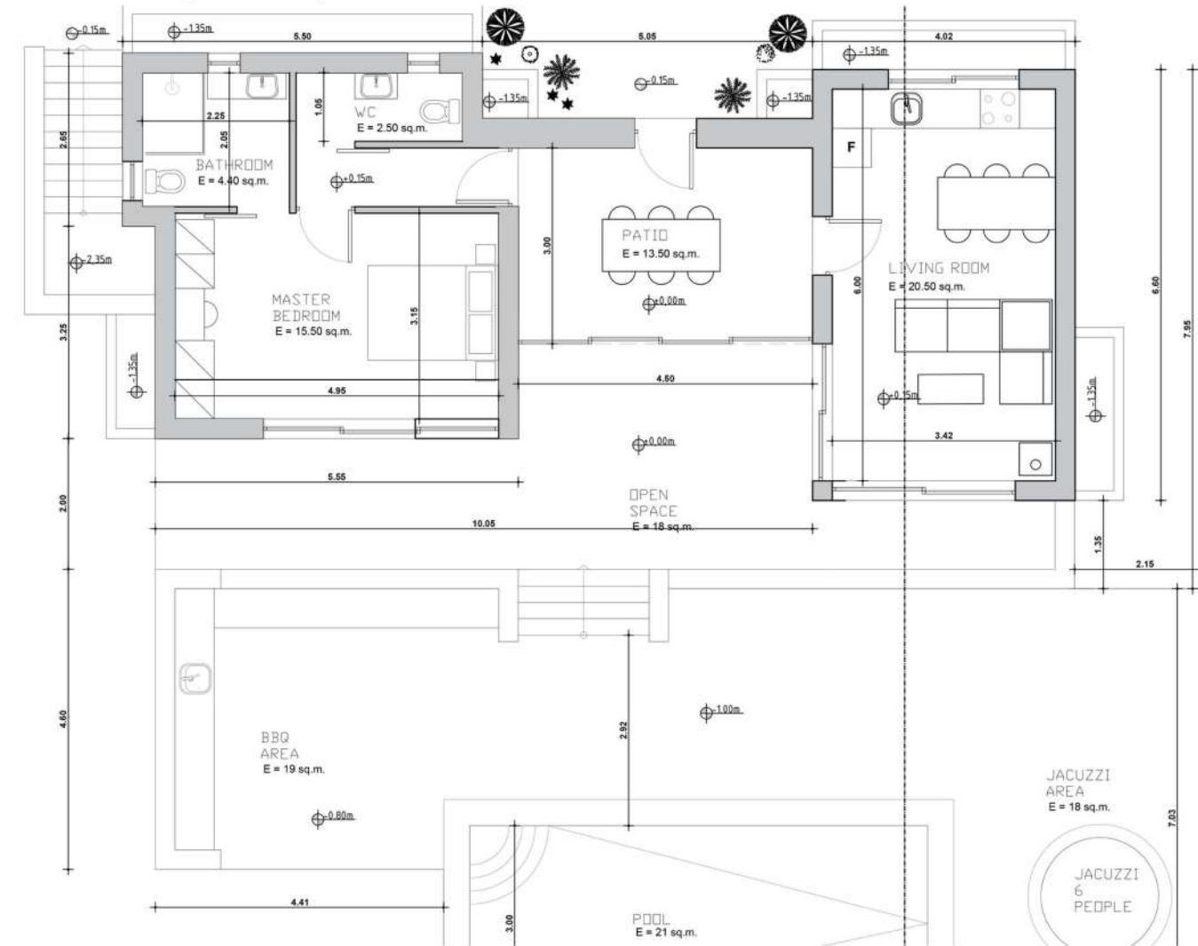
Plan : plain-pied - 73m 2
