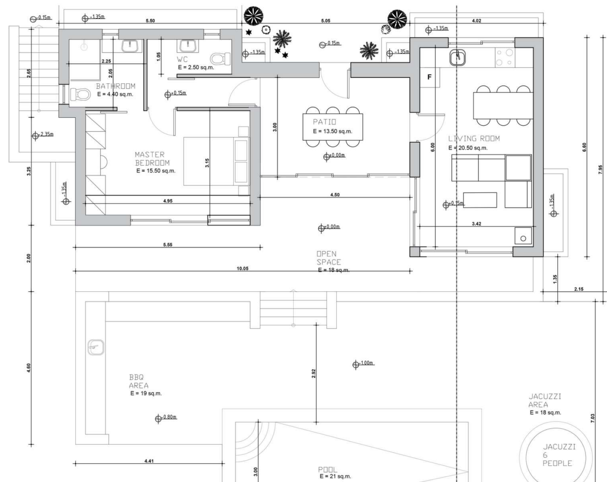
PLAN VILLA 1
